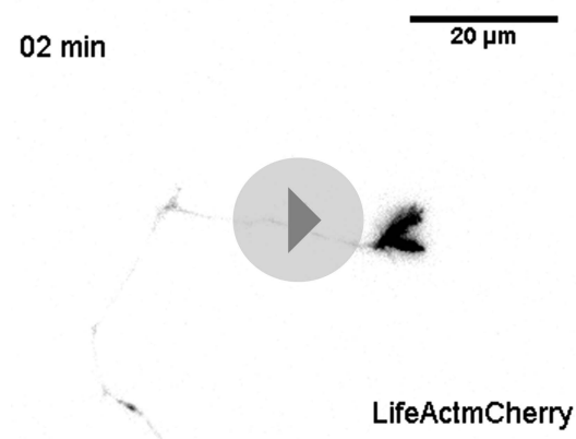
Video 3. Effect of actin depolymerization on CB1R-induced growth cone retraction. Dynamic, F-actin-rich growth cone of a cultured hippocampal neuron co-expressing CB1R-eCFP, LifeAct-mCherry, and EB3-eGFP at DIV6 pre-treated with 1 \mu M cytochalasin D at 20 min before treatment with 100 nM WIN at 40 min. Scale bar: 20 \mu m. DOI: 10.7554/eLife.03159.014
